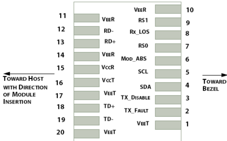
Figure 2: Interface to Host PCB
