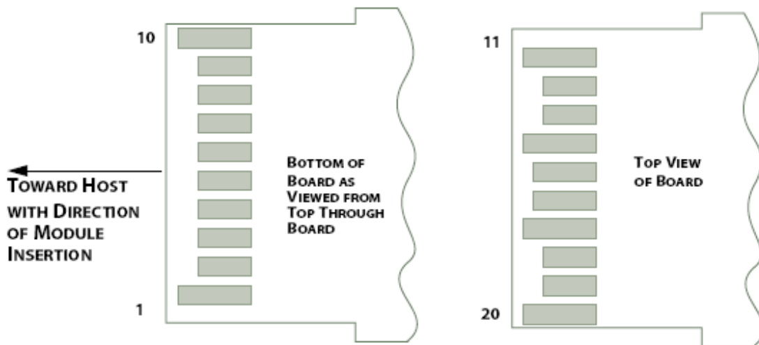
Figure 3: Module Contact Assignment
