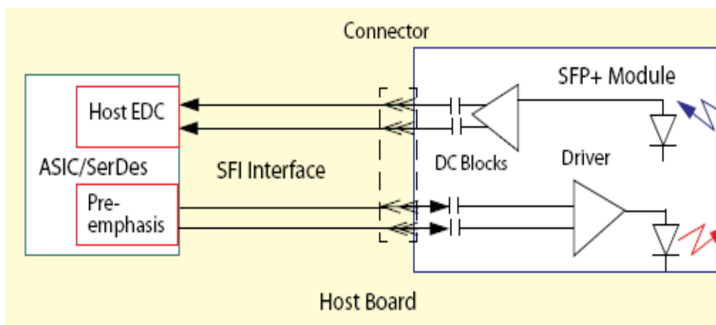
Figure 1: Interface to Host
